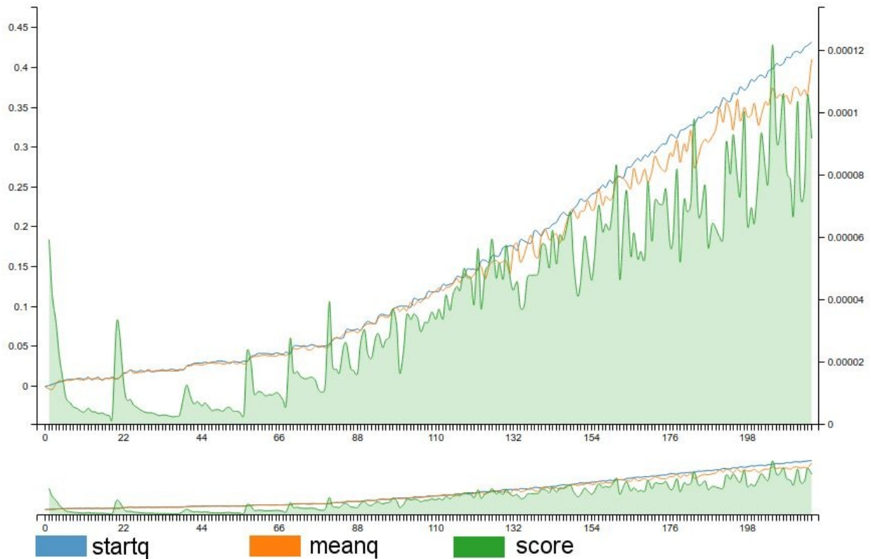
Figure B-10. Score and mean-Q graph
