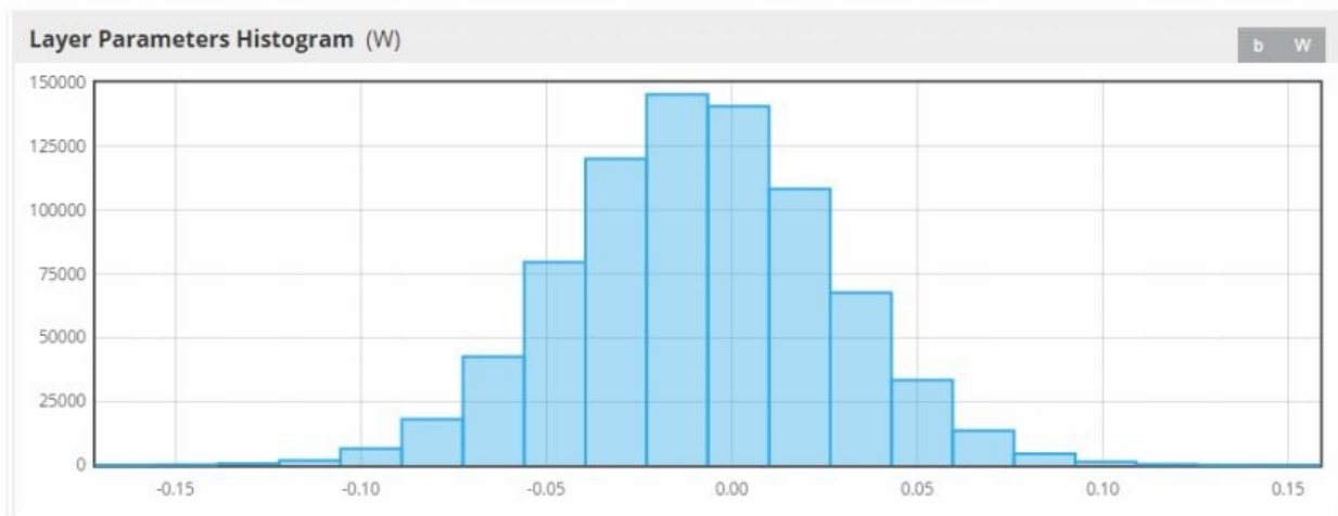
Figure 6-11. Layer Parameters Histogram panel with normal weights
