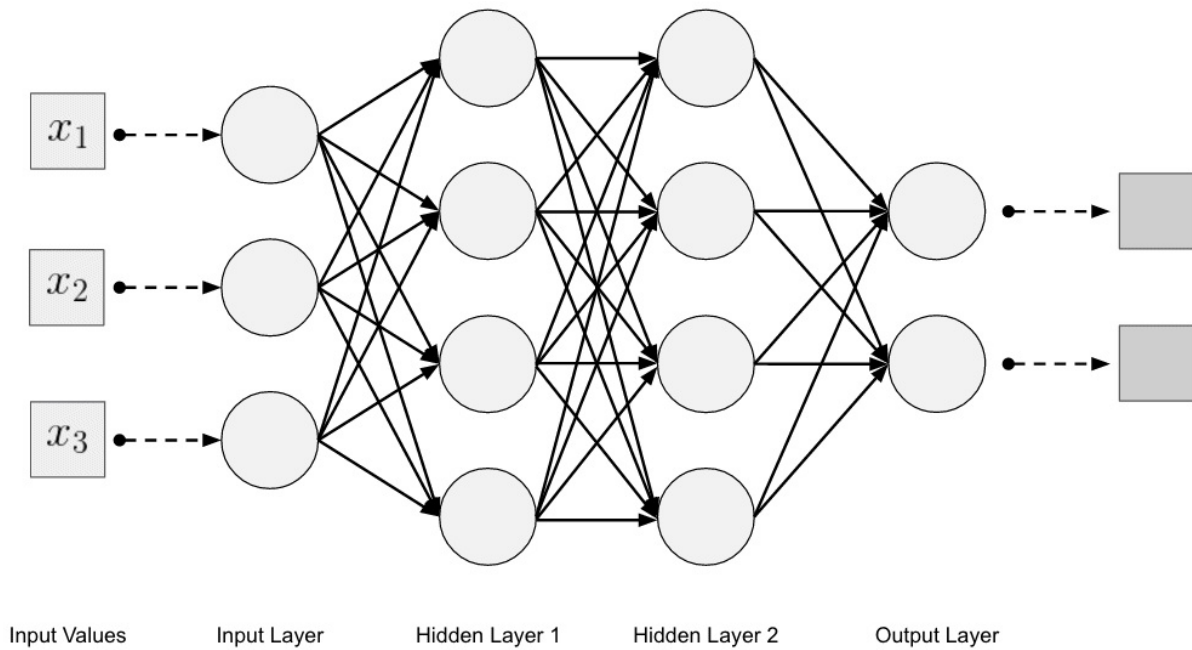
Figure 2-1. Multilayer neural network topology
