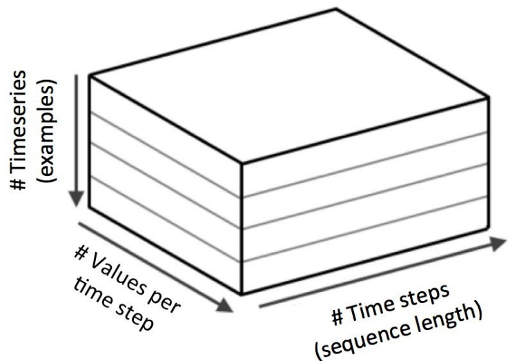
Figure 4-17. Normal input vectors compared to recurrent neural networks input
