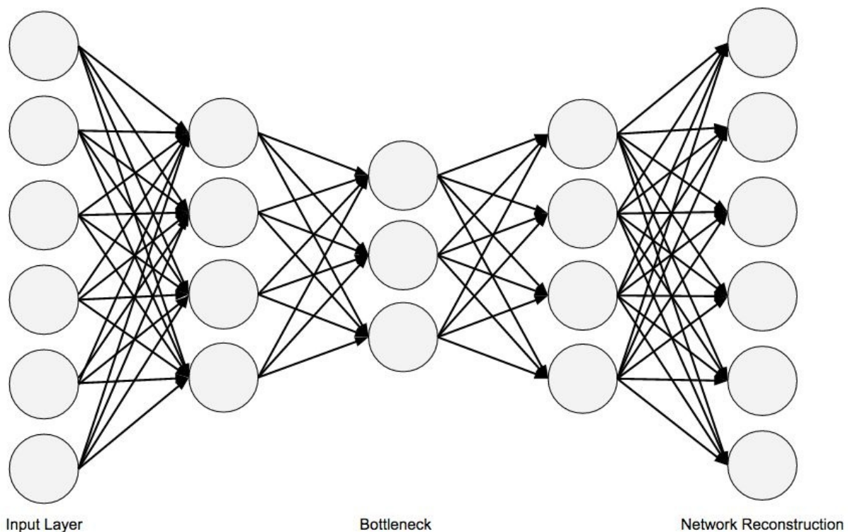
Figure 3-7. Autoencoder network architecture
