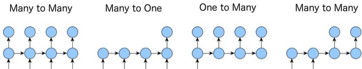
Figure 7-3. Different variations of Recurrent Neural Network training
