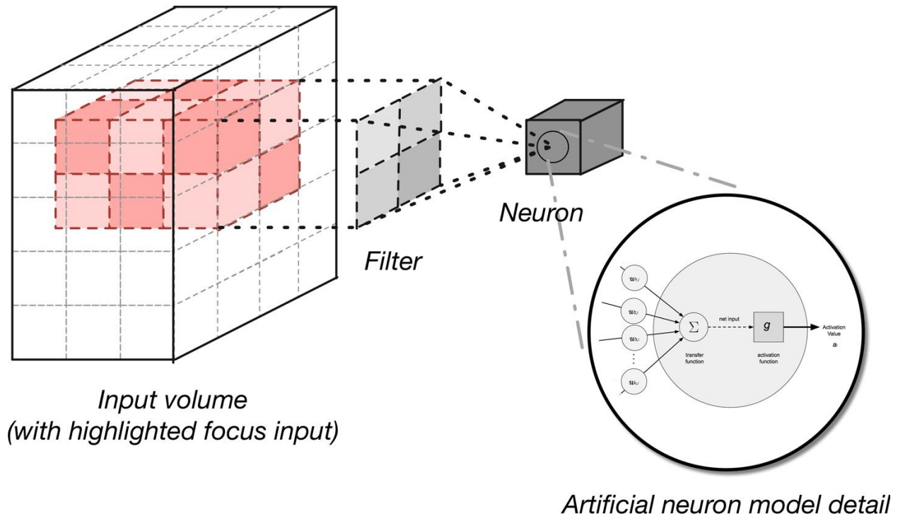
Figure 4-15. Generating an activation output volume
