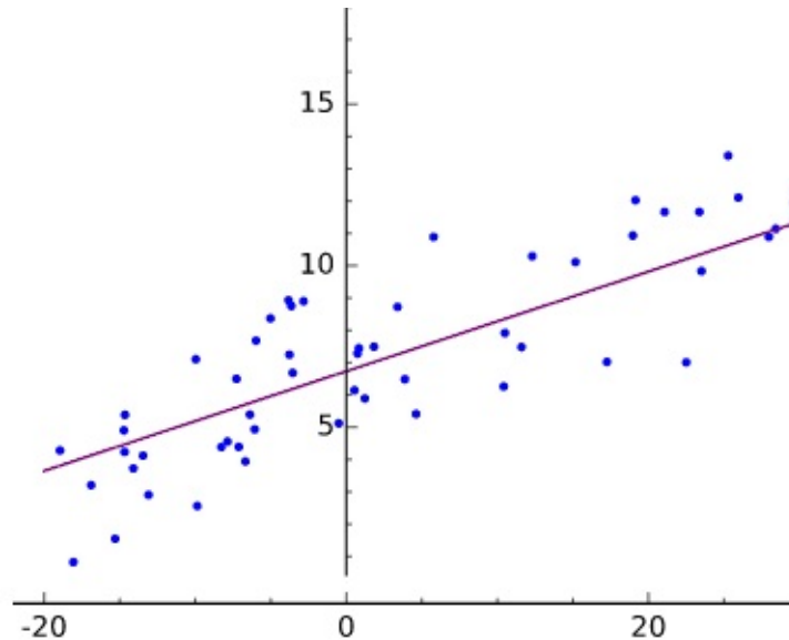
Figure 1-6. Linear regression plotted
