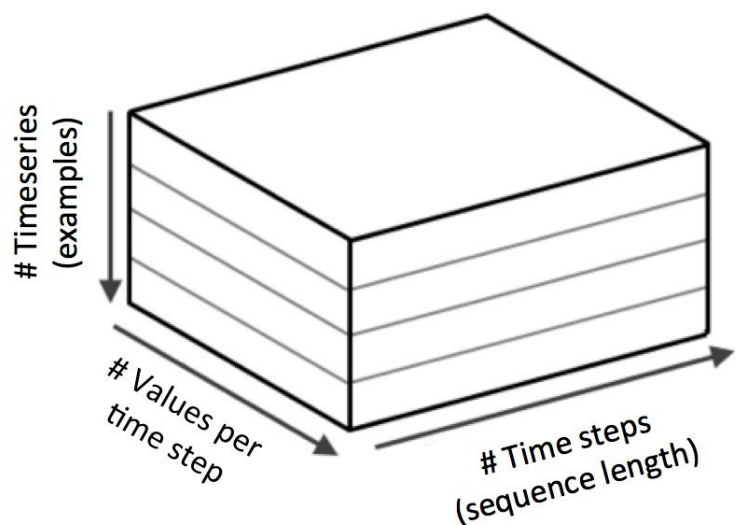
Figure 8-2. Representing sequential data for Recurrent Neural Networks
