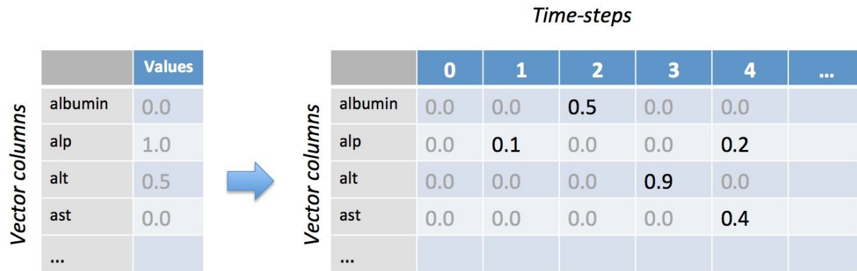
Figure 4-18. The time-step aspect of Recurrent Neural Network input
