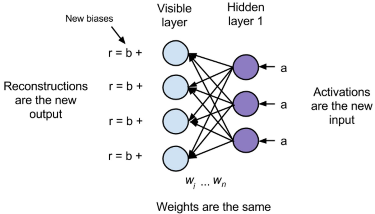
Figure 3-4. Reconstruction in RBMs
