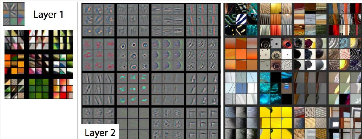
Figure 4-5. Visualizing deconvolutional layers
