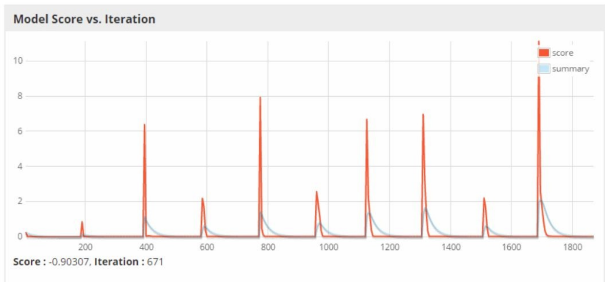
Figure 6-9. Training model scores with spikes
