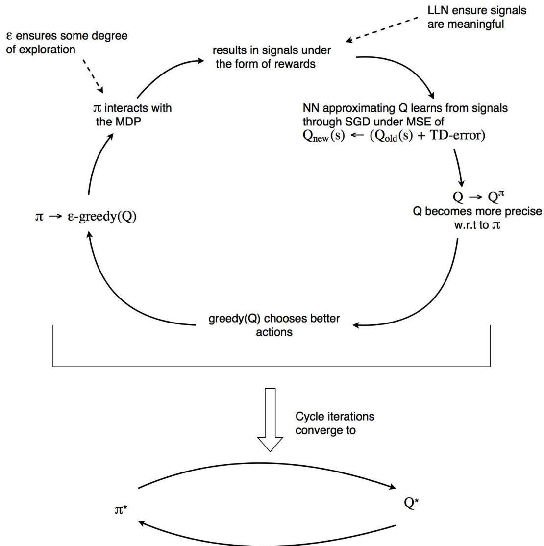
Figure B-4. Policy iteration
