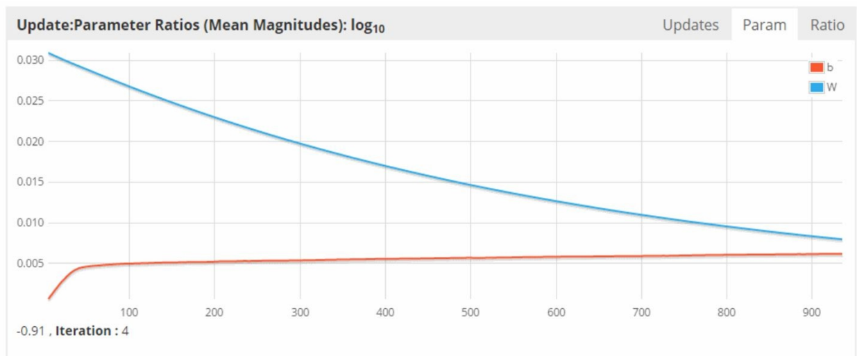
Figure 6-10. Weight values falling toward zero on the UI
