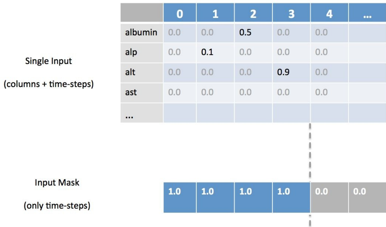
Figure 4-19. Masking specific time-steps
