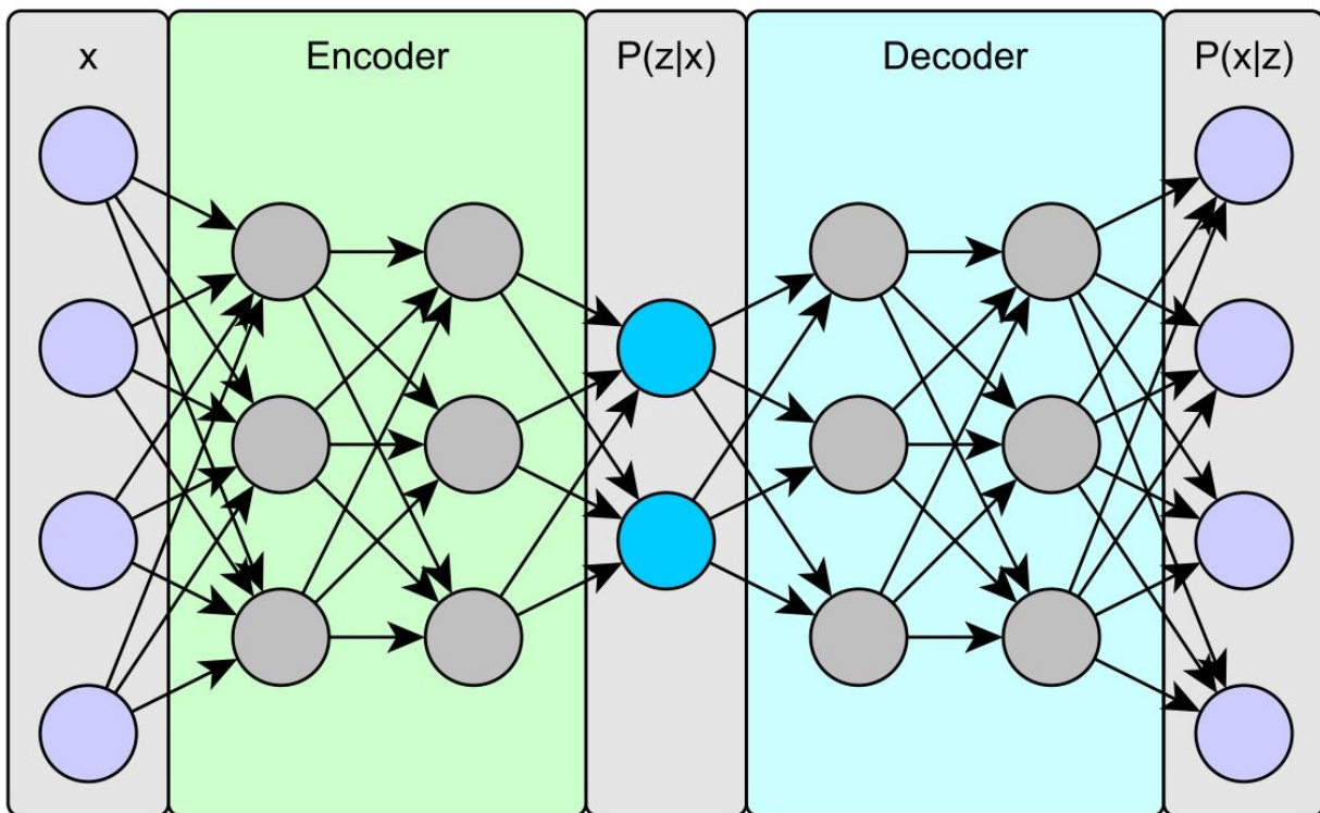
Figure 3-8. VAE network architecture
