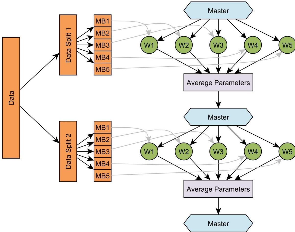
Figure 6-3. DL4J's Parameter averaging parallelization strategy
