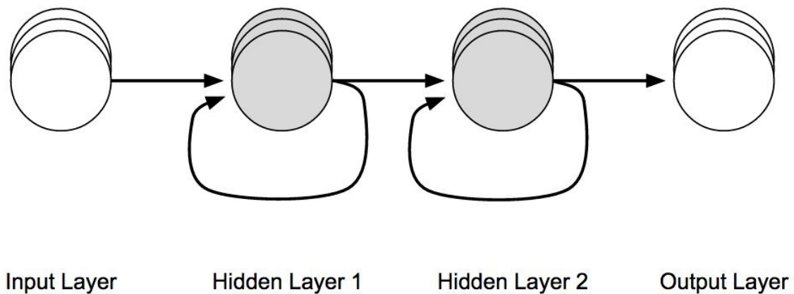
Figure 4-22. Showing recurrent connections on hidden-layer nodes
