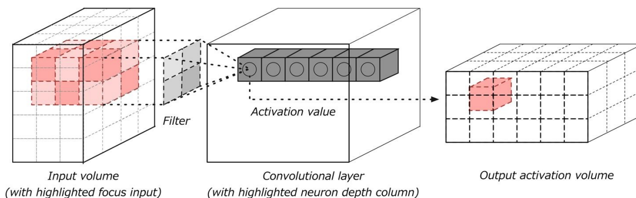
Figure 4-11. Convolution layer with input and output volumes
