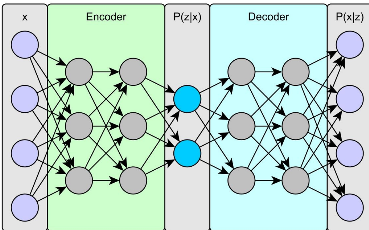
Figure 5-5. VAE network architecture
