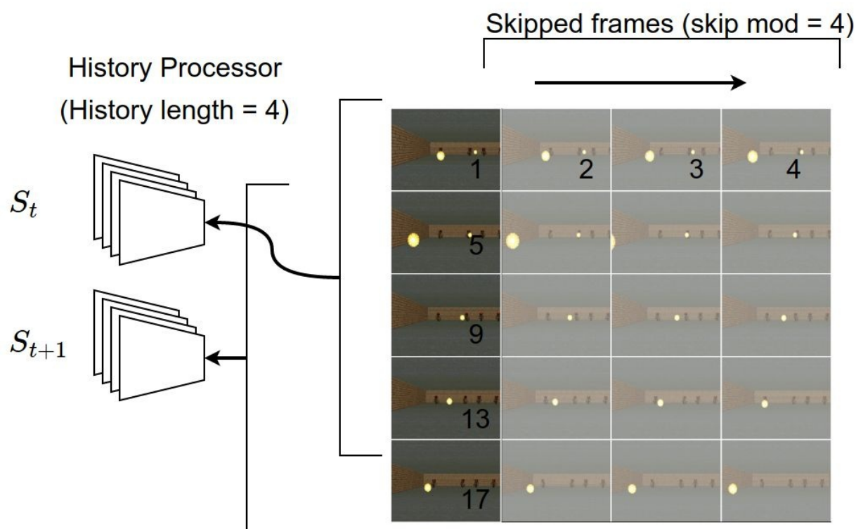
Figure B-7. History processing and stacking
