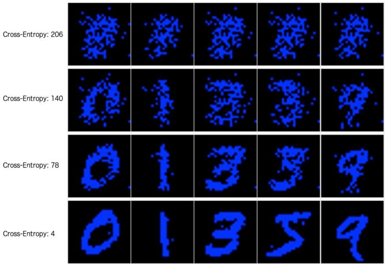
Figure 3-6. Reconstructing MNIST digits with RBMs
