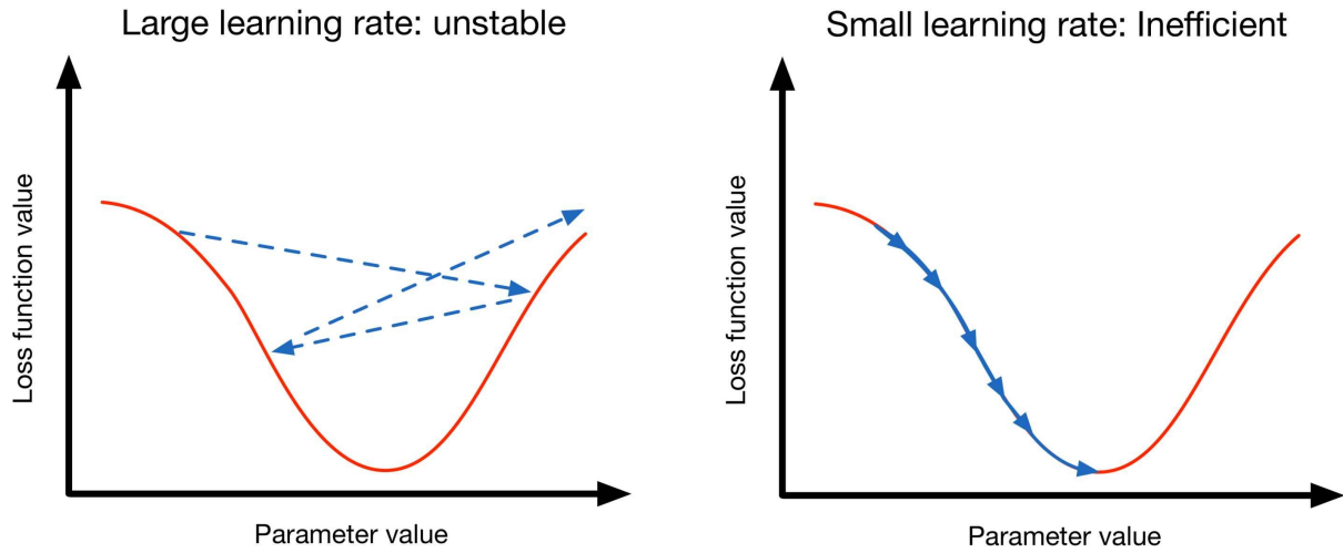
Figure 6-1. SGD and learning rate
