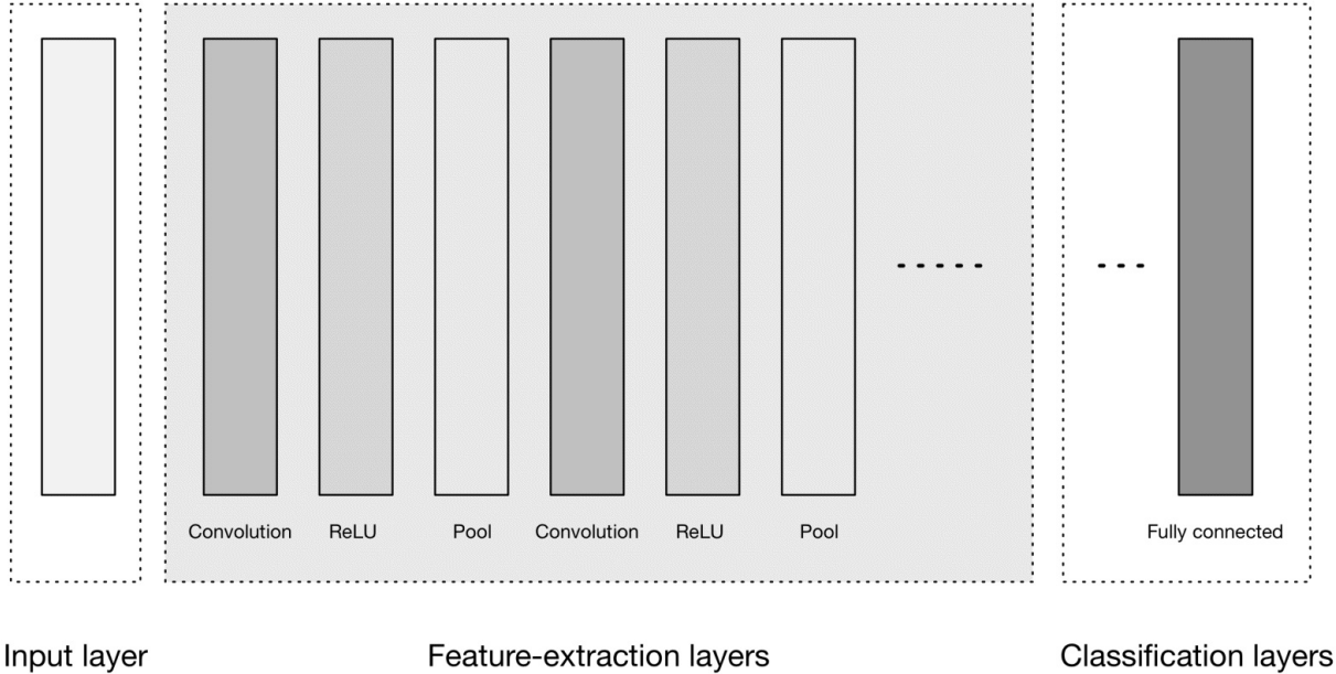
Figure 4-9. High-level general CNN architecture
