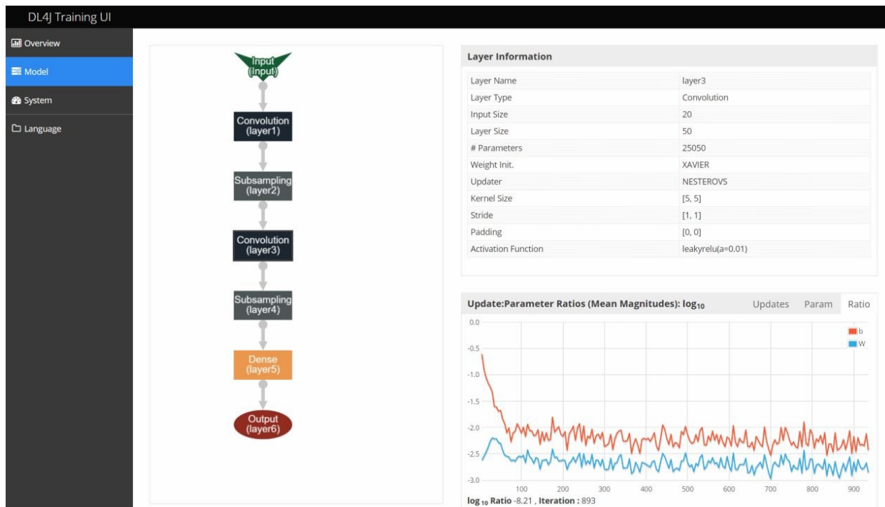
Figure 6-5. The DL4J training UI Model page
