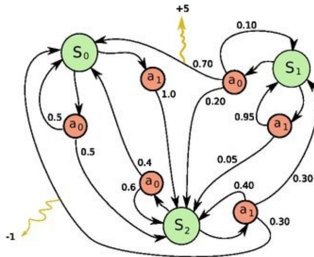
Figure B-1. Schema of an MDP
