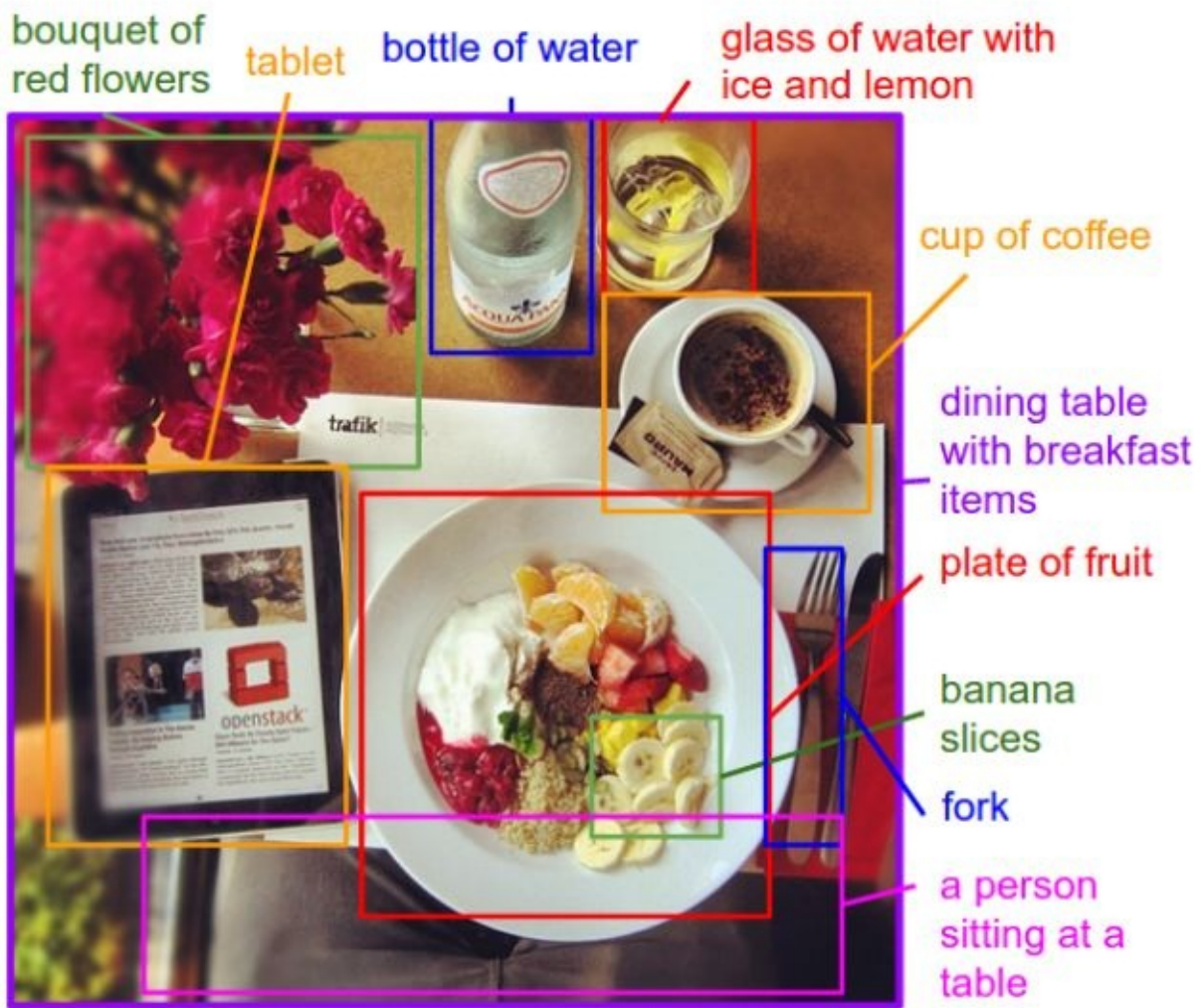
Figure 4-28. Labeling images with a blended CNN/Recurrent Neural Network 38
