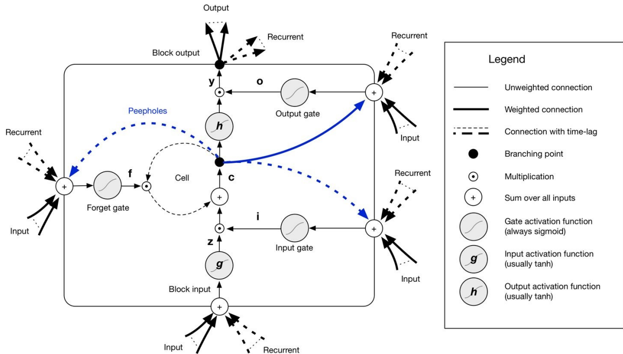
Figure 4-24. LSTM block diagram
