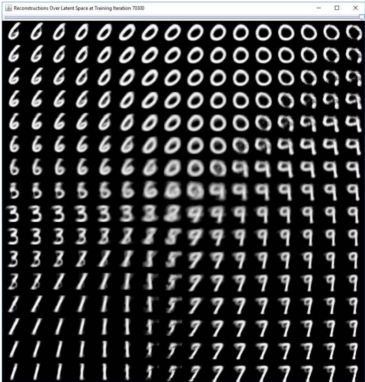
Figure 5-4. MNIST digits generated by the VAE example
