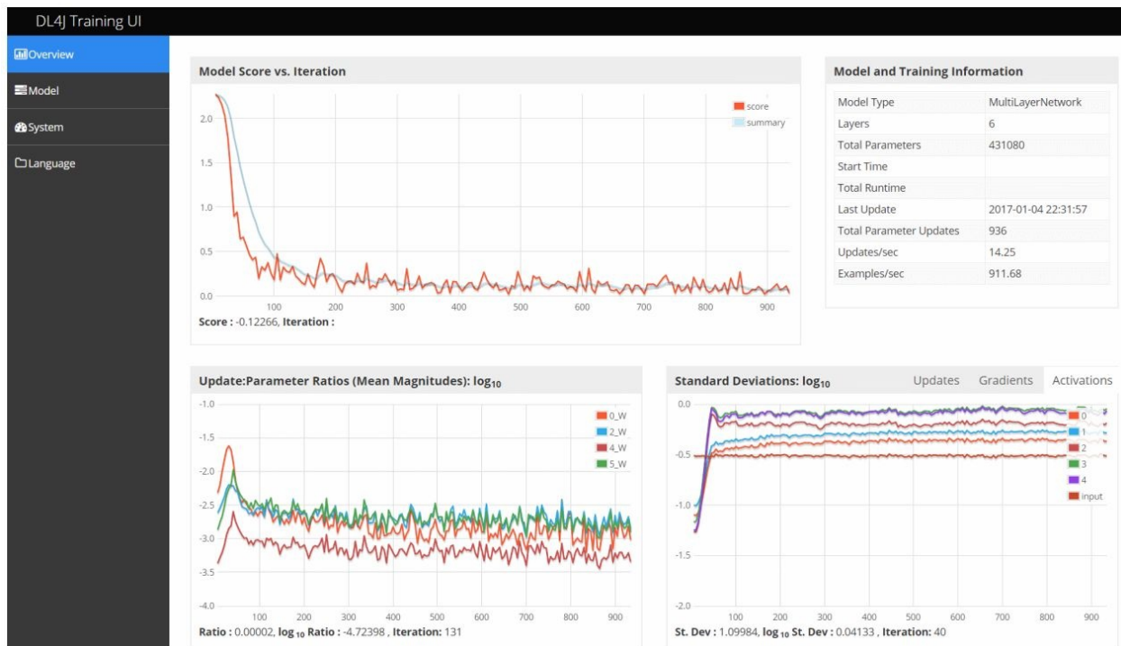
Figure 6-4. The DL4J network statistics tool
