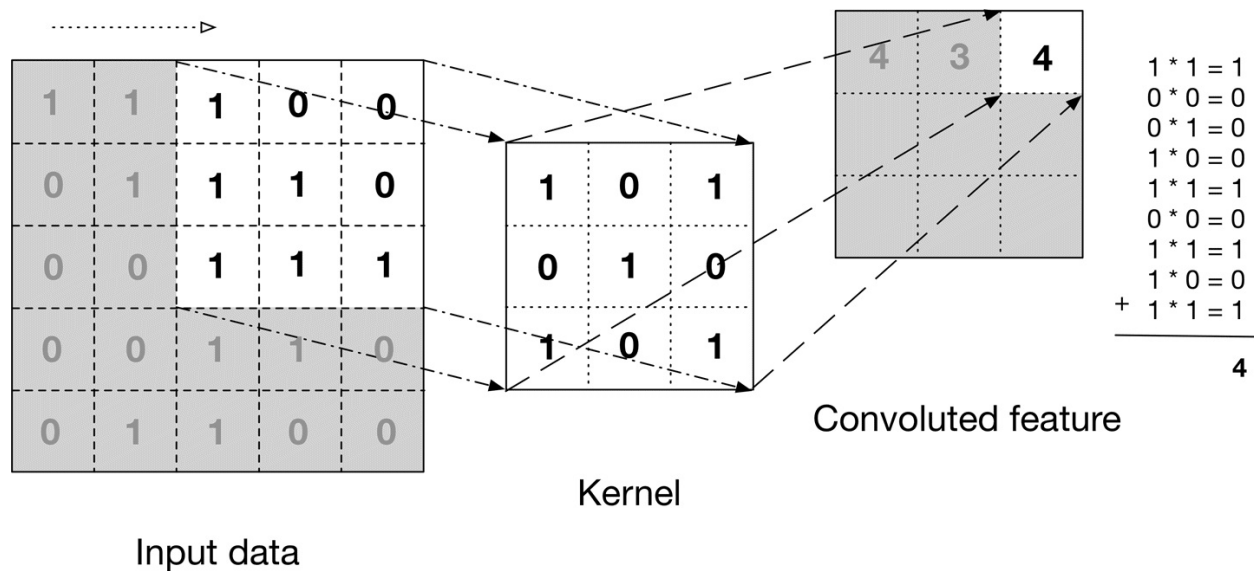
Figure 4-12. The convolution operation
