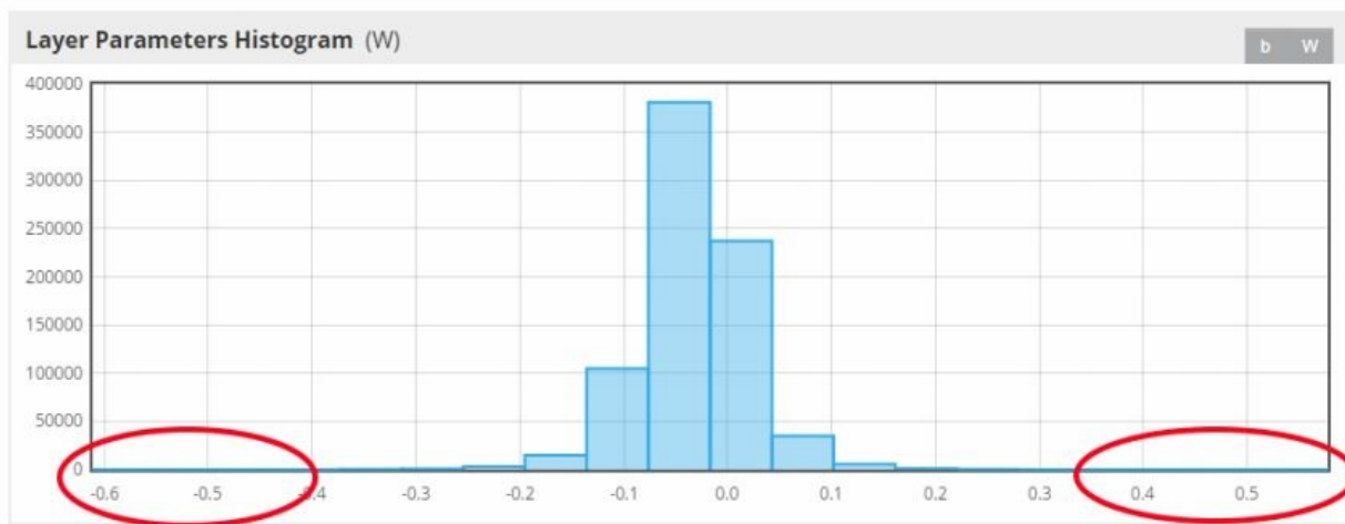
Figure 6-12. Layer Parameters Histogram with a few large weights
