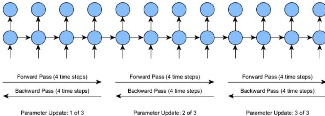
Figure 4-27. Truncated BPTT
