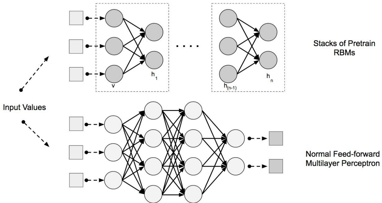
Figure 4-1. DBN architecture
