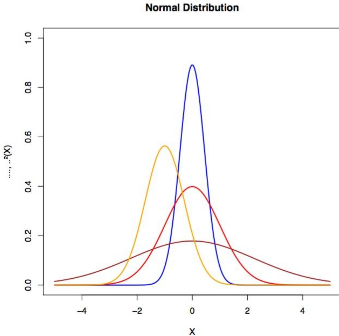
Figure 1-5. Examples of normal distributions
