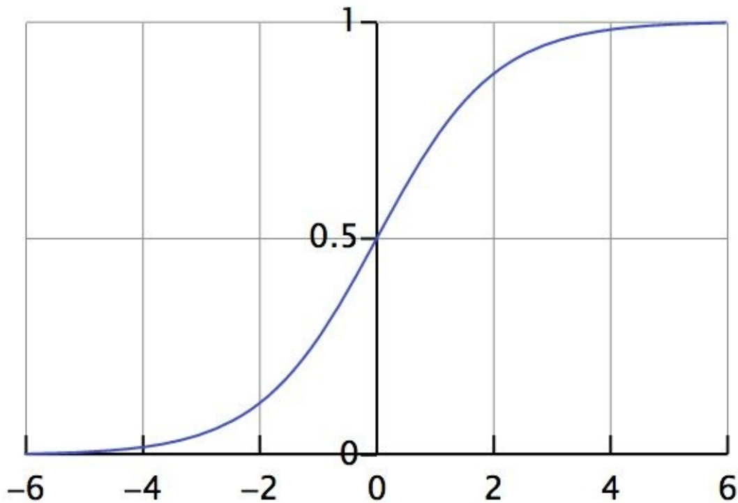
Figure 1-10. Plot of the logistic function
