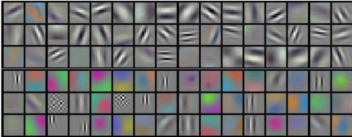
Figure 4-16. Example filters learned by Krizhevsky et al. 10 (96 filters, 11 \times 11 \times 3 )
