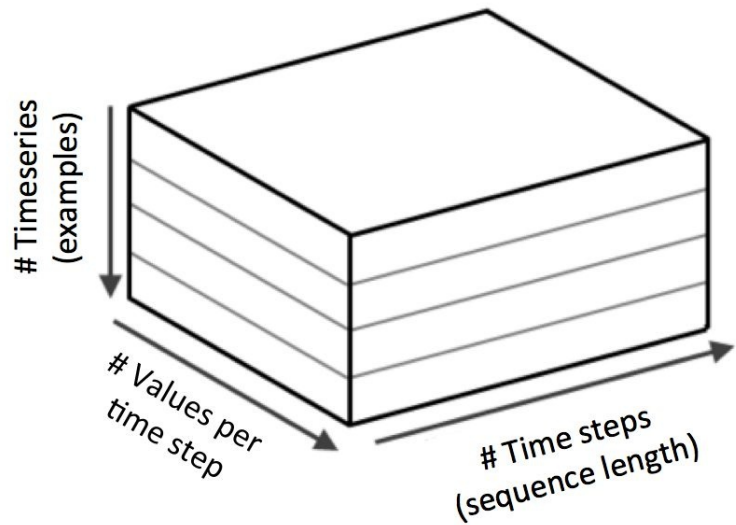
Figure 7-2. Representing 3D input for Recurrent Neural Networks
