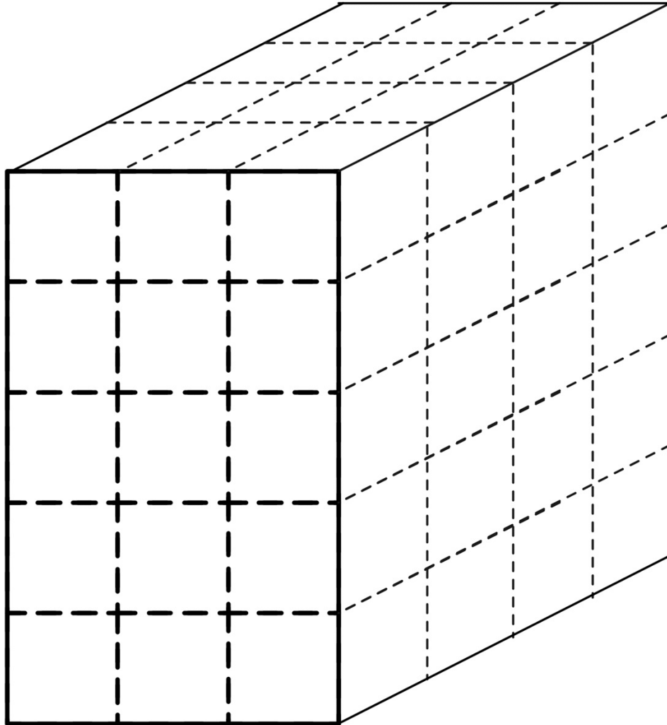
Figure 4-10. Input layer 3D volume
