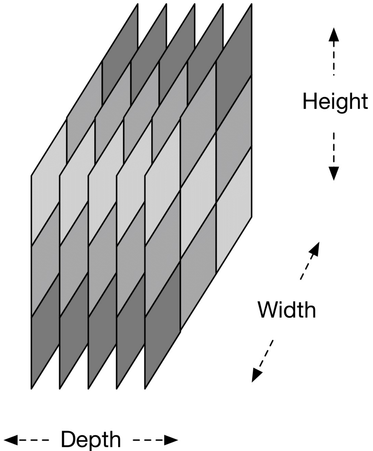
Figure 4-14. Activation volume output of convolutional layer
